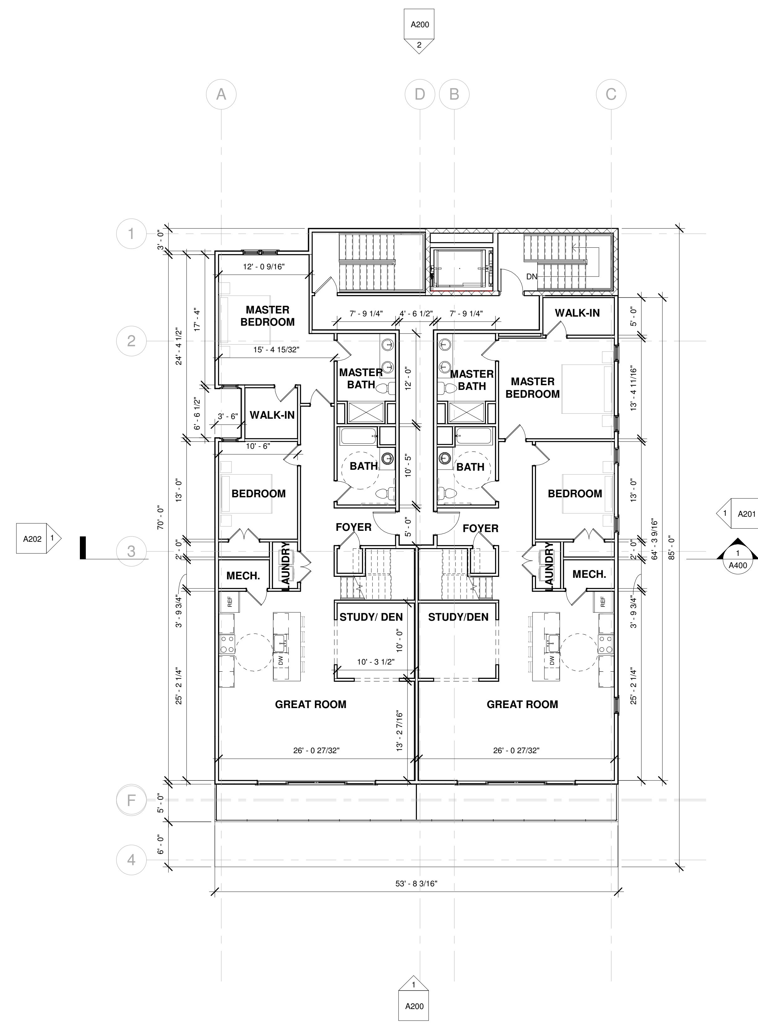
1 RESIDENTIAL LEVEL 3 1/8" = 1'-0"
