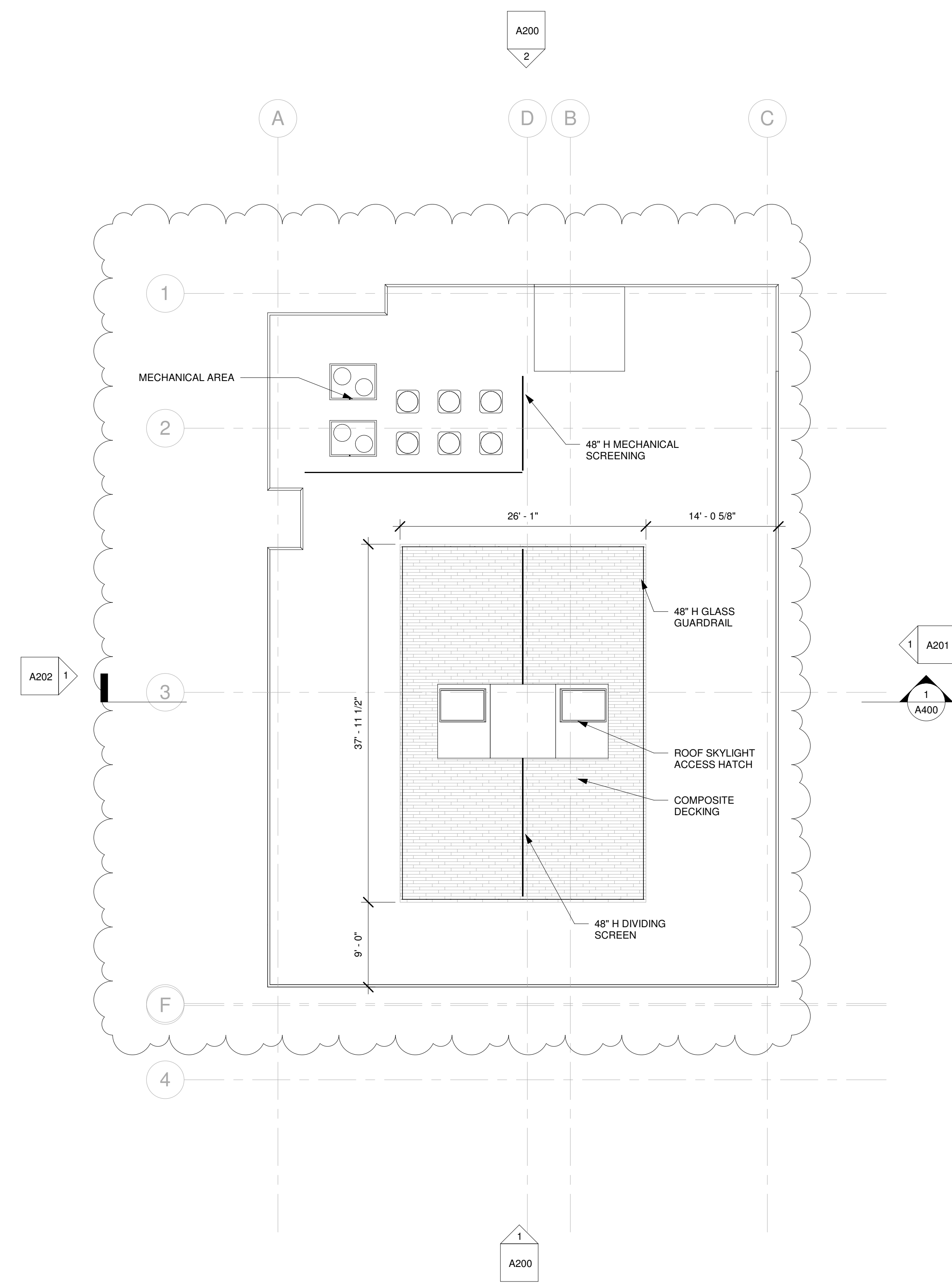
2 ROOF 1/8" = 1'-0"
