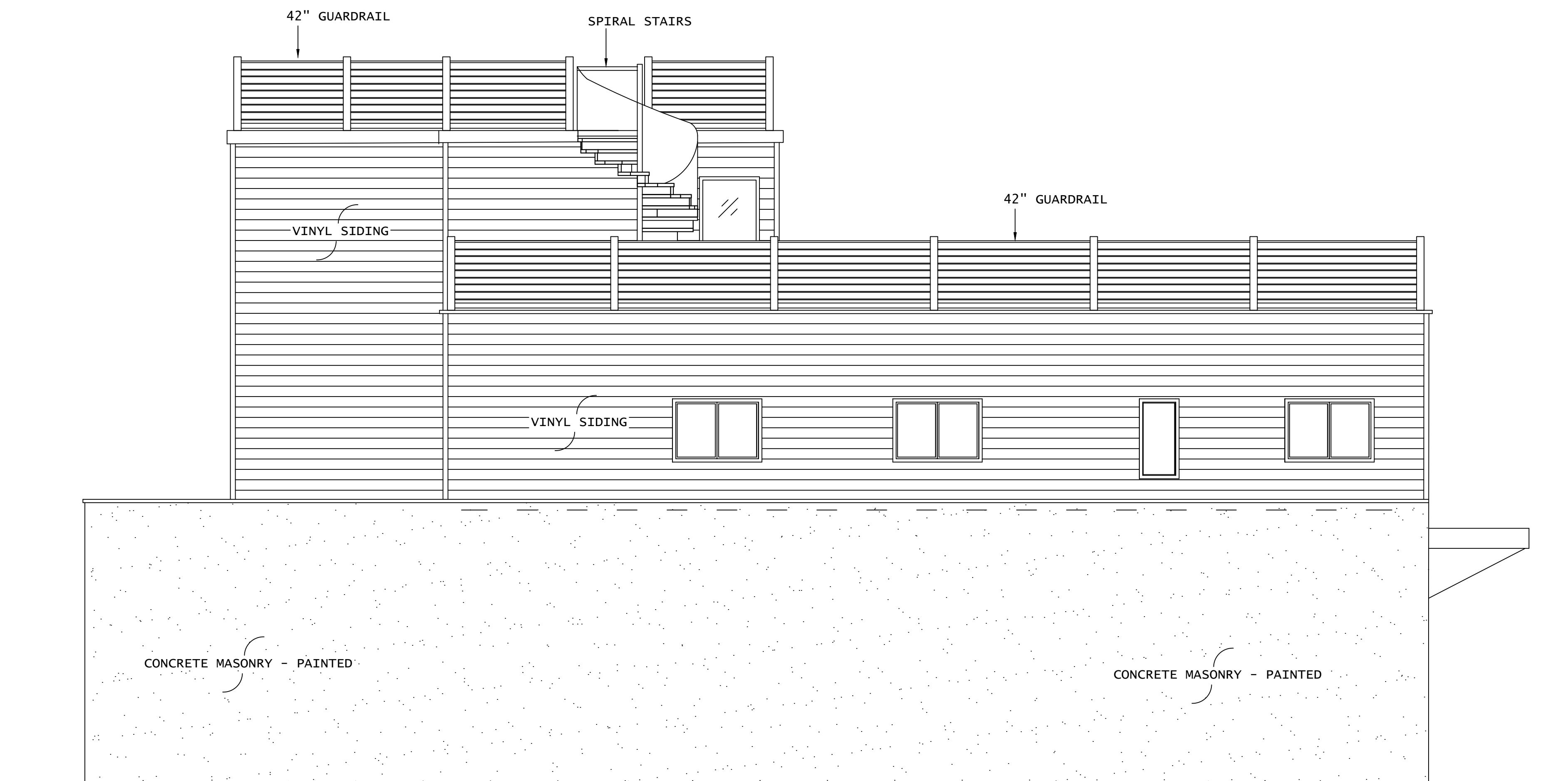
PROPOSED SOUTH ELEVATION 1/4"=1'-0"
