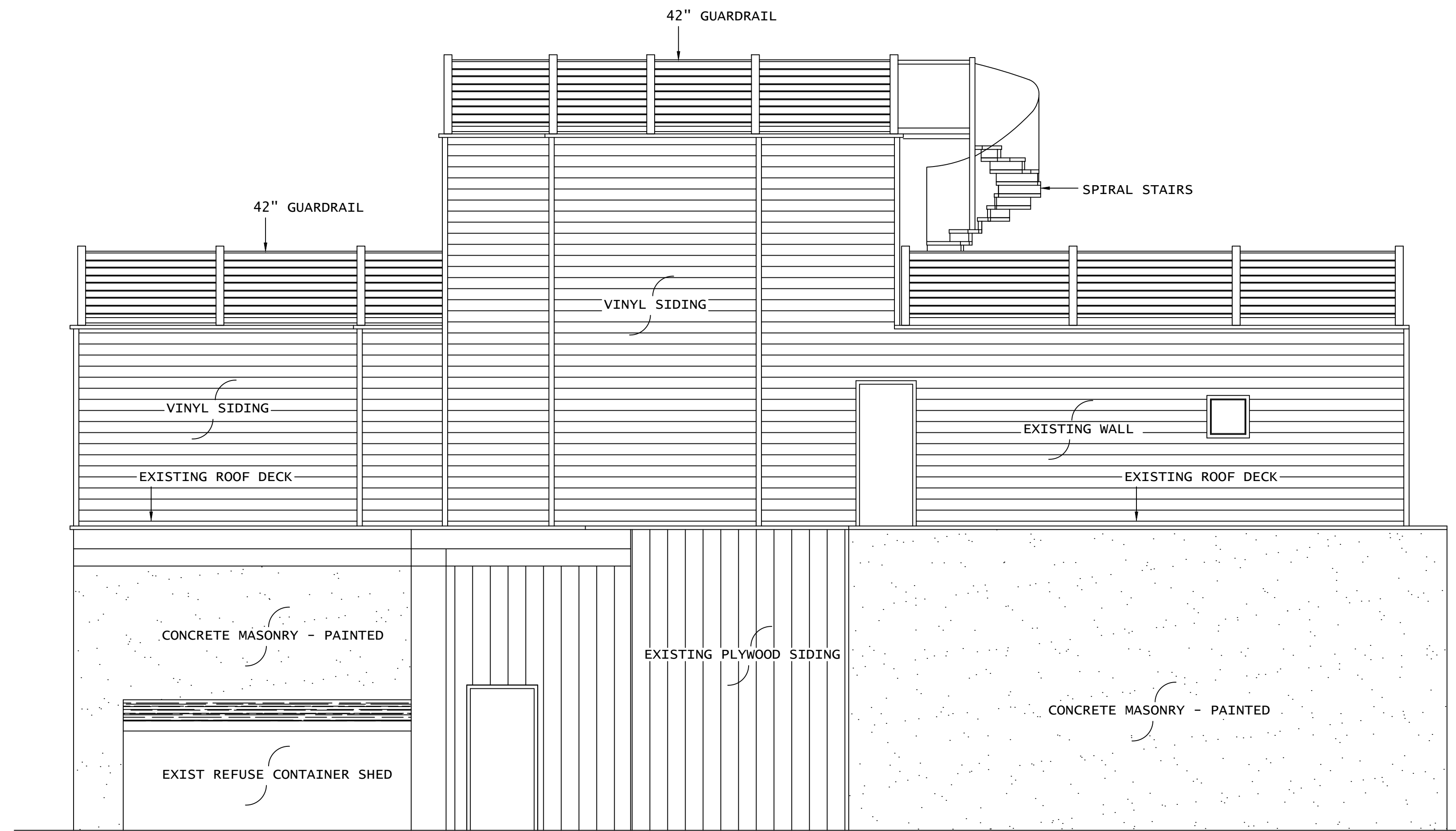
PROPOSED WEST ELEVATION 1/4"=1'-0"
